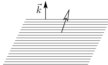
extraordinary ray
