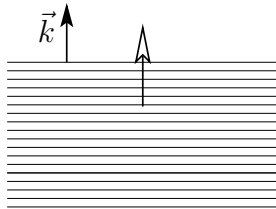
ordinary ray
