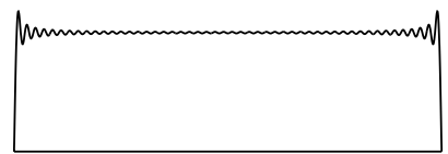
highest harmonic: 99
